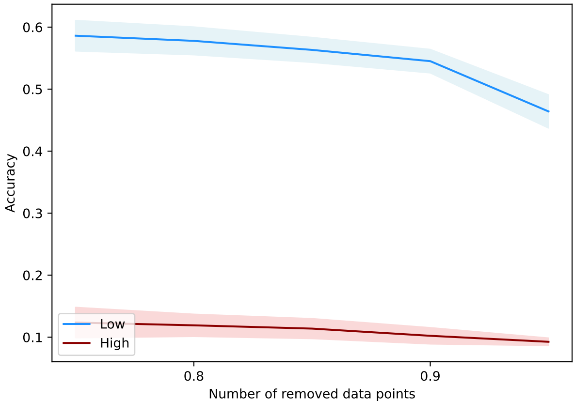
DataAttrOpt(10000, 0.03, 15, best, +b, alpha=best) - cifar10-embedding
